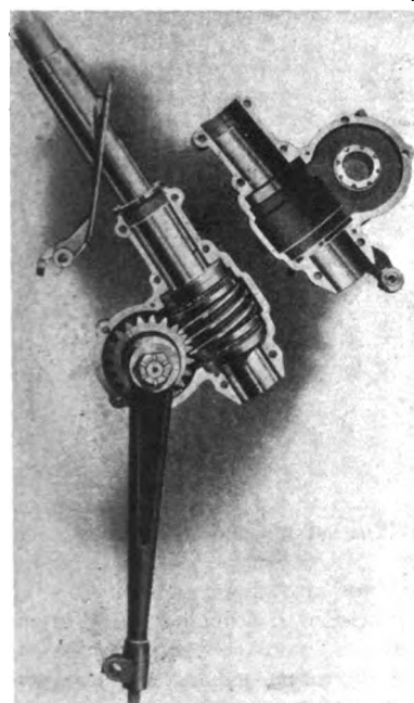
Ball Bearing Worm and Gear Peerless Steering Device.
